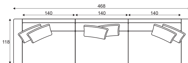
6S - seater
