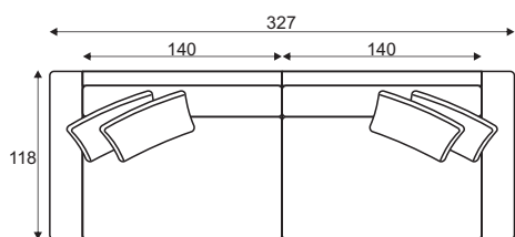
4S - seater
